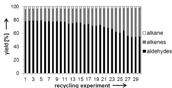
Figure 2. Catalyst recycling in the hydroformylation of 1-dodecene in 30 consecutive experiments.
