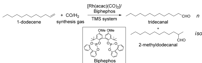
Scheme 1. The hydroformylation of 1-dodecene.
